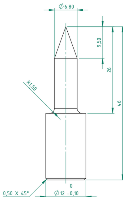
SHORT PIN
